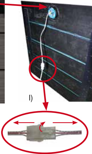
Disconnect logo light wire from back side of door panel
